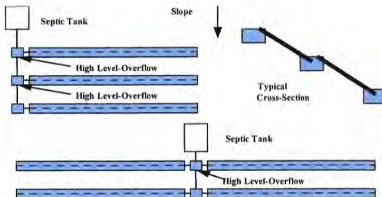
Figure 9 - Serial Distribution Systems
