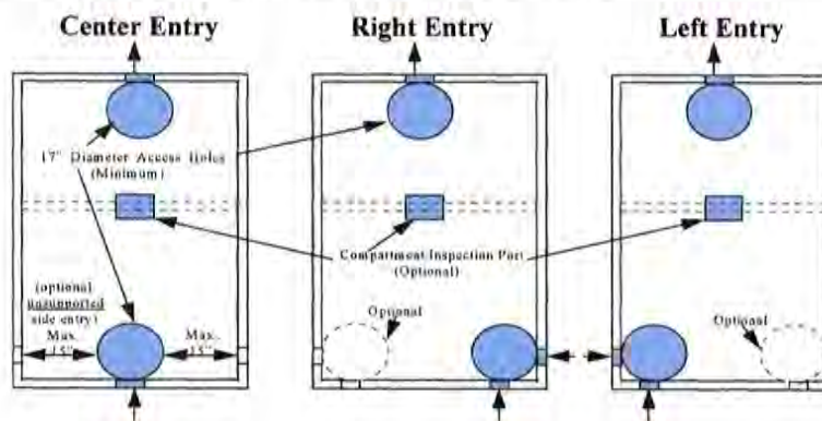
Figure 6 – Standard Septic Tank Configurations
