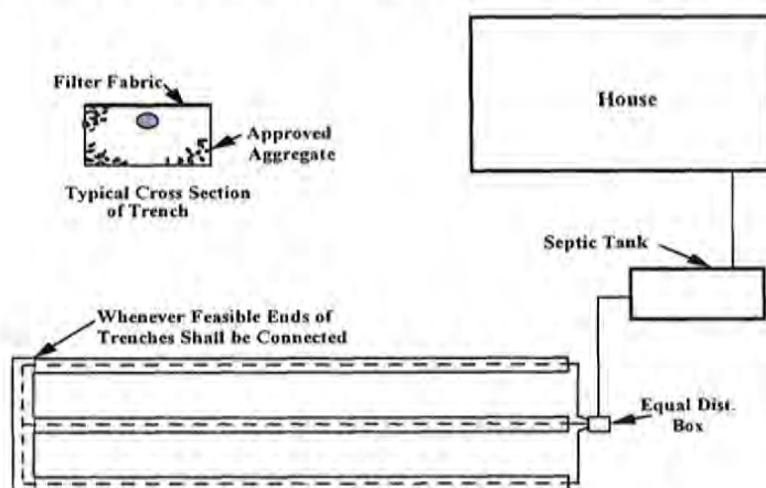
Figure 8 - Level Leaching Systems
