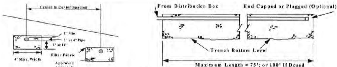
Figure 14 - Leaching Trenches
