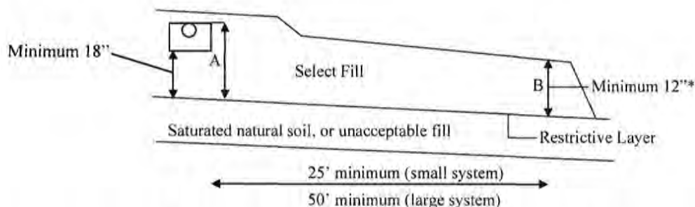
Diagram 6 – Select Fill Receiving Soil (Sloped Restrictive Layer)
