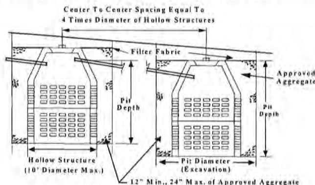
Figure 15 - Leaching Pits
