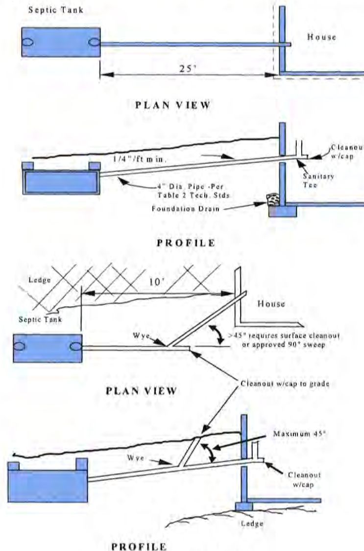
Figure 1 - Building Sewers
