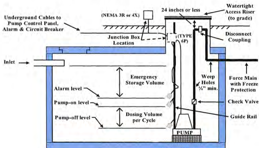
Figure 11 - Pump Chamber
