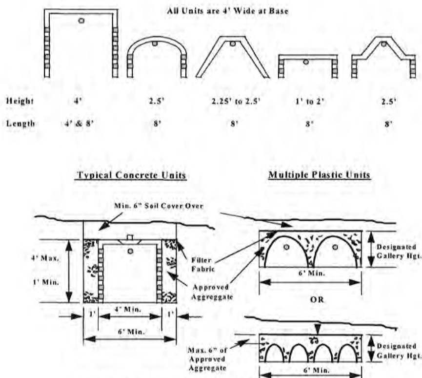
Figure 16 - Typical Leaching Gallery Structures
